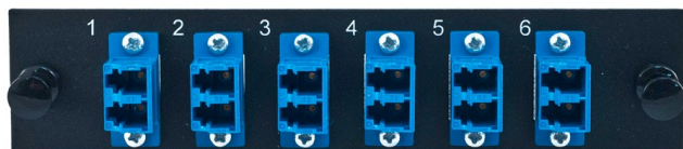
6 x LC Duplex OS2 UPC
