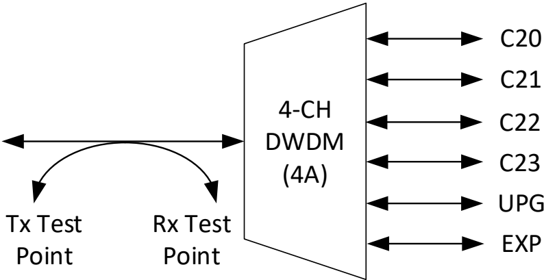
4-Channel DWDM Design (high level)
